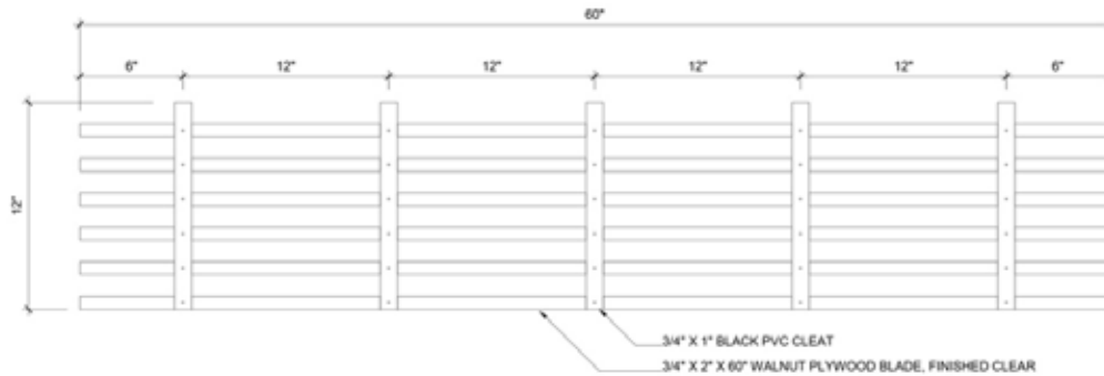
SIX BLADE ASSEMBLY EXAMPLE (TOP VIEW)
