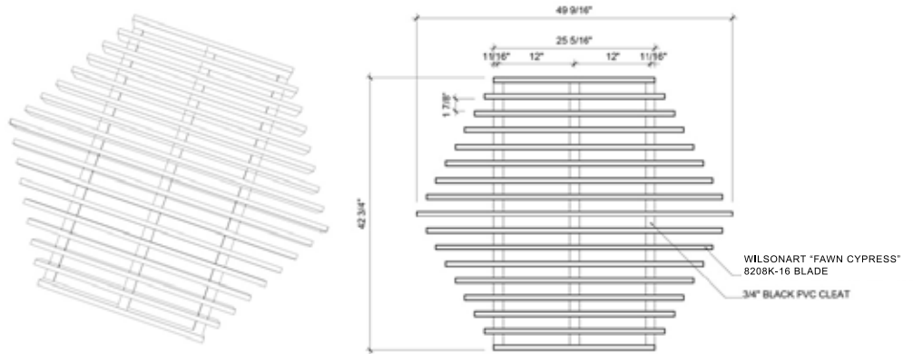
EXAMPLE CUSTOM BLADE ASSEMBLY (TOP VIEW)
