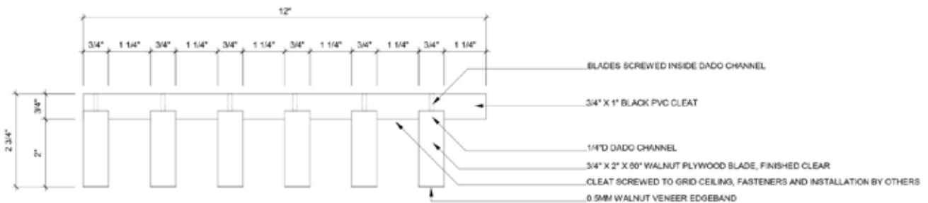
SIX BLADE ASSEMBLY EXAMPLE (END VIEW)
